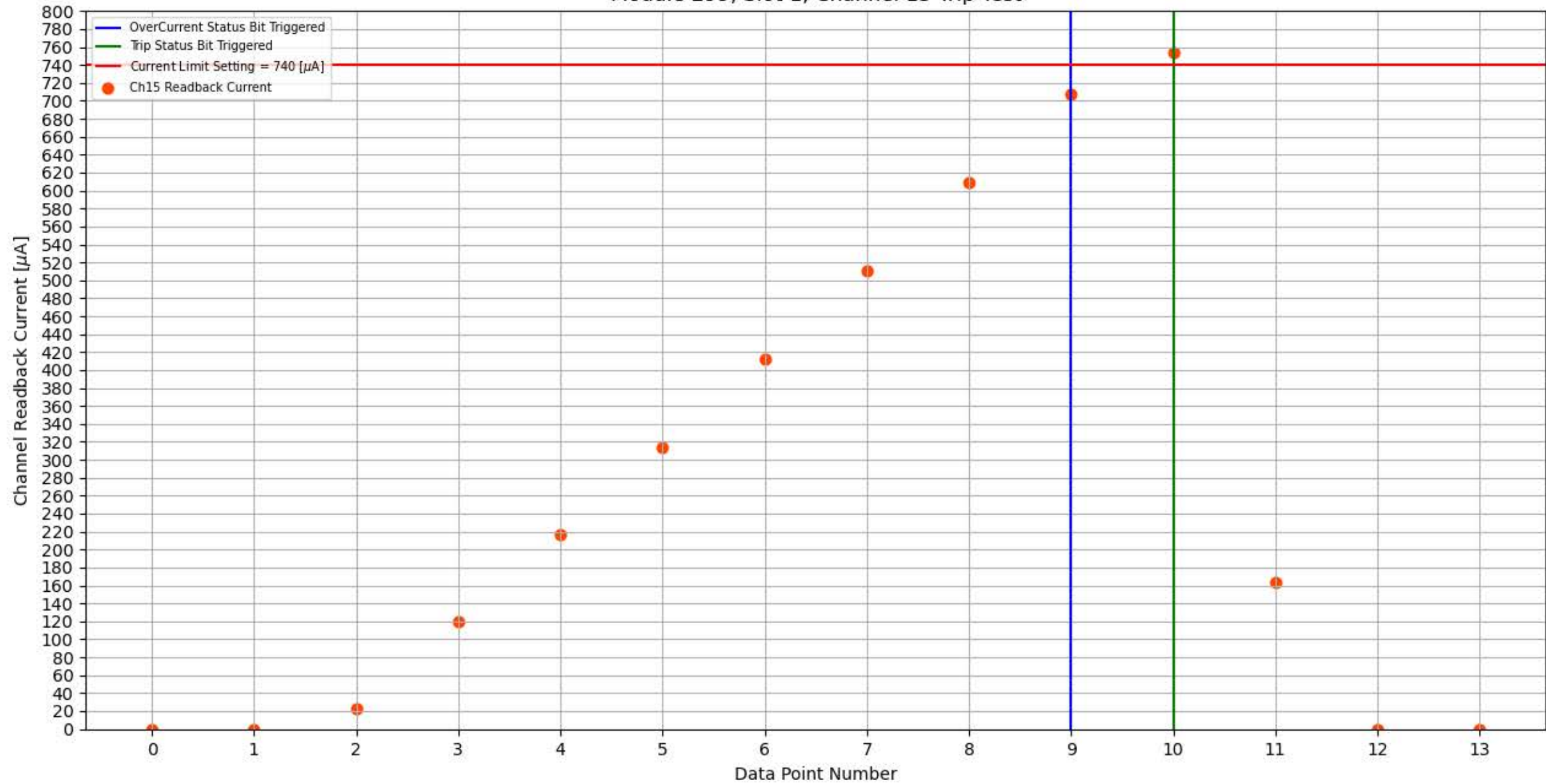
Module 299, Slot 1, Channel 15 Trip Test
