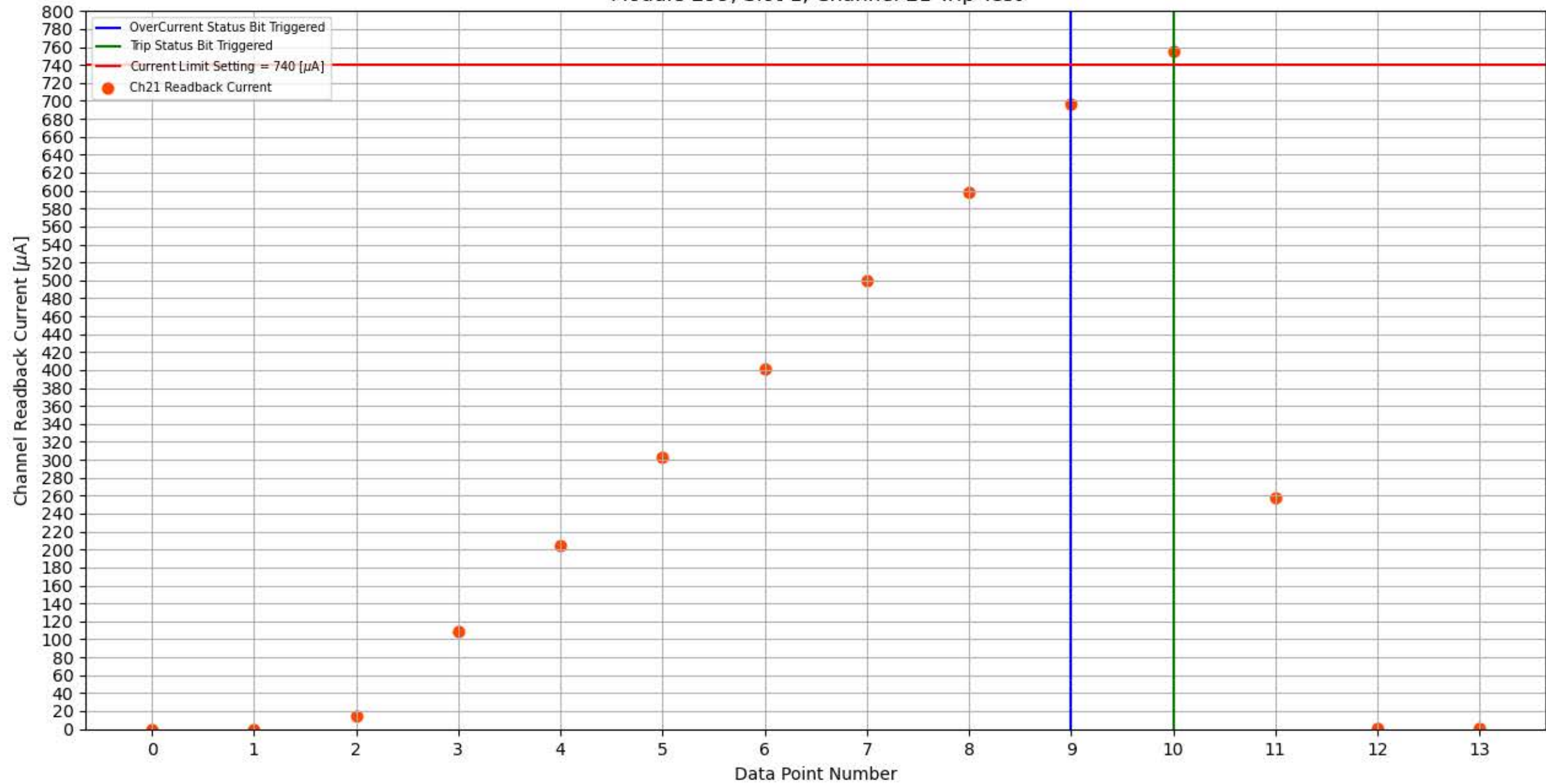
Module 299, Slot 1, Channel 21 Trip Test
