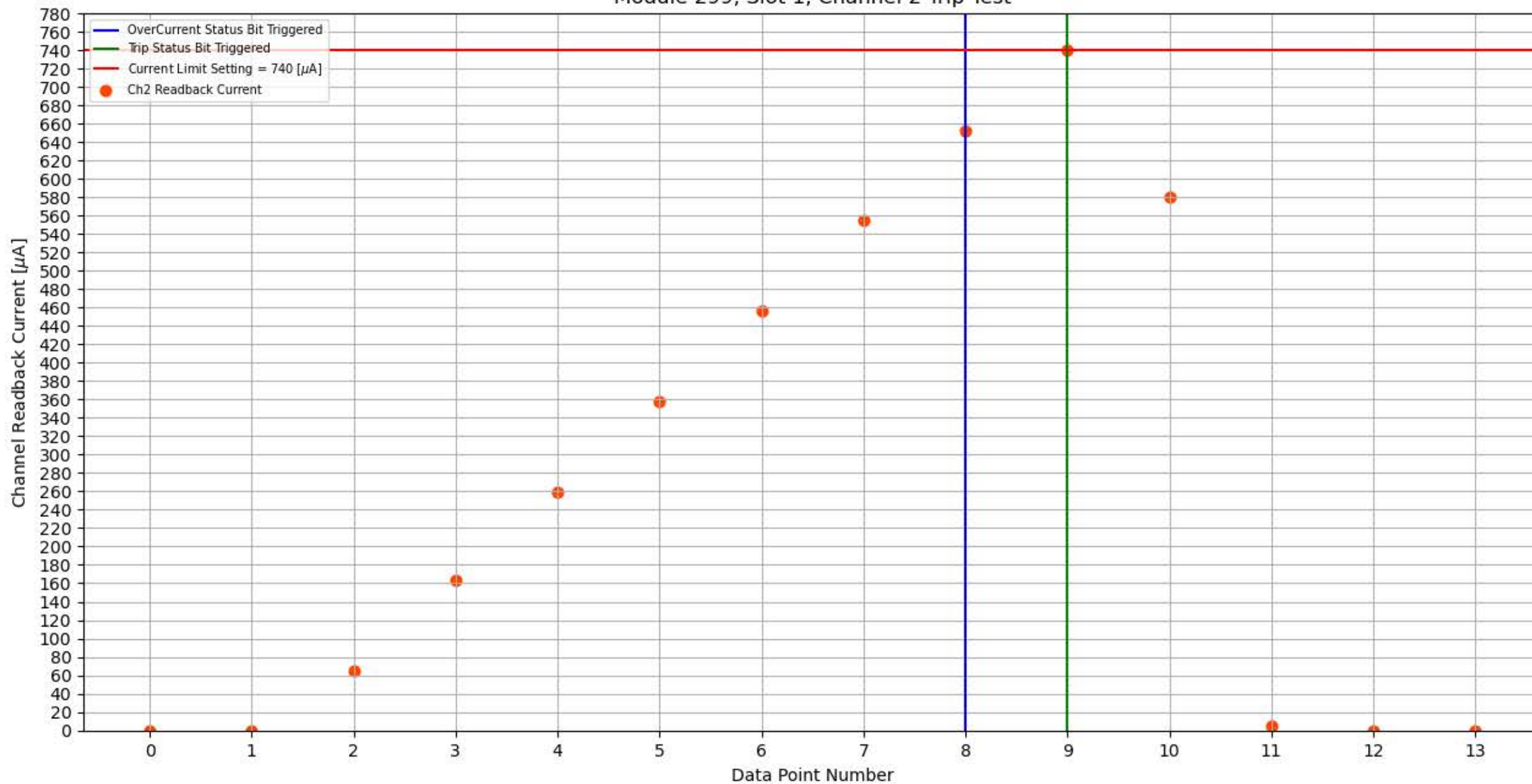
Module 299, Slot 1, Channel 2 Trip Test
