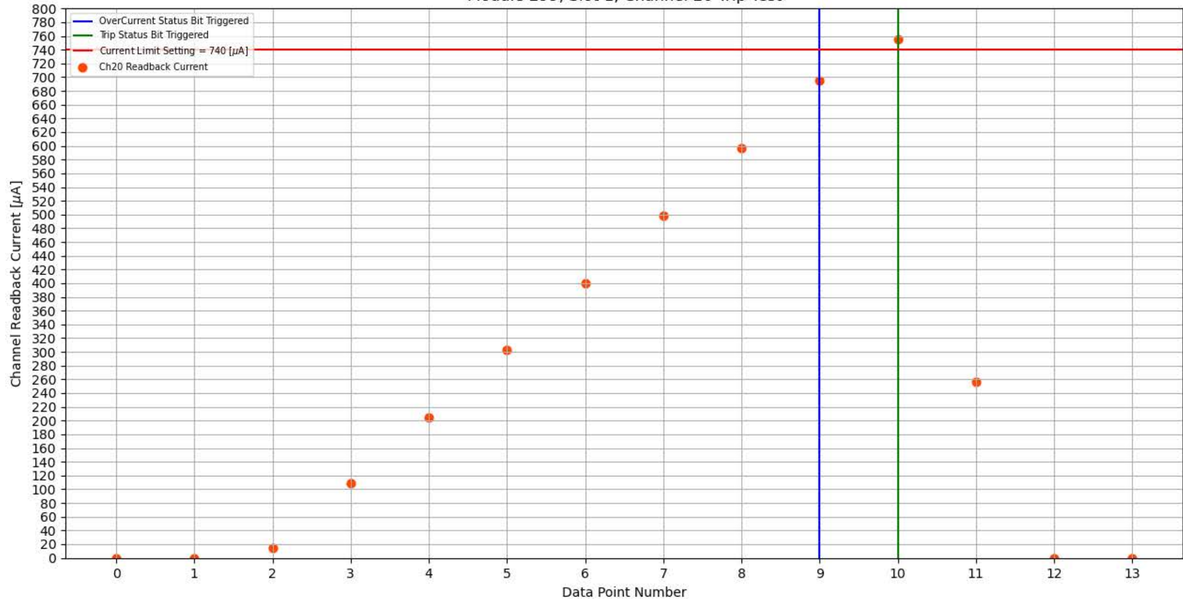
Module 299, Slot 1, Channel 20 Trip Test
