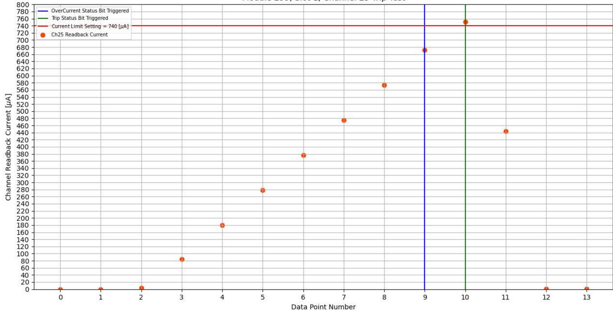
Module 299, Slot 1, Channel 25 Trip Test
