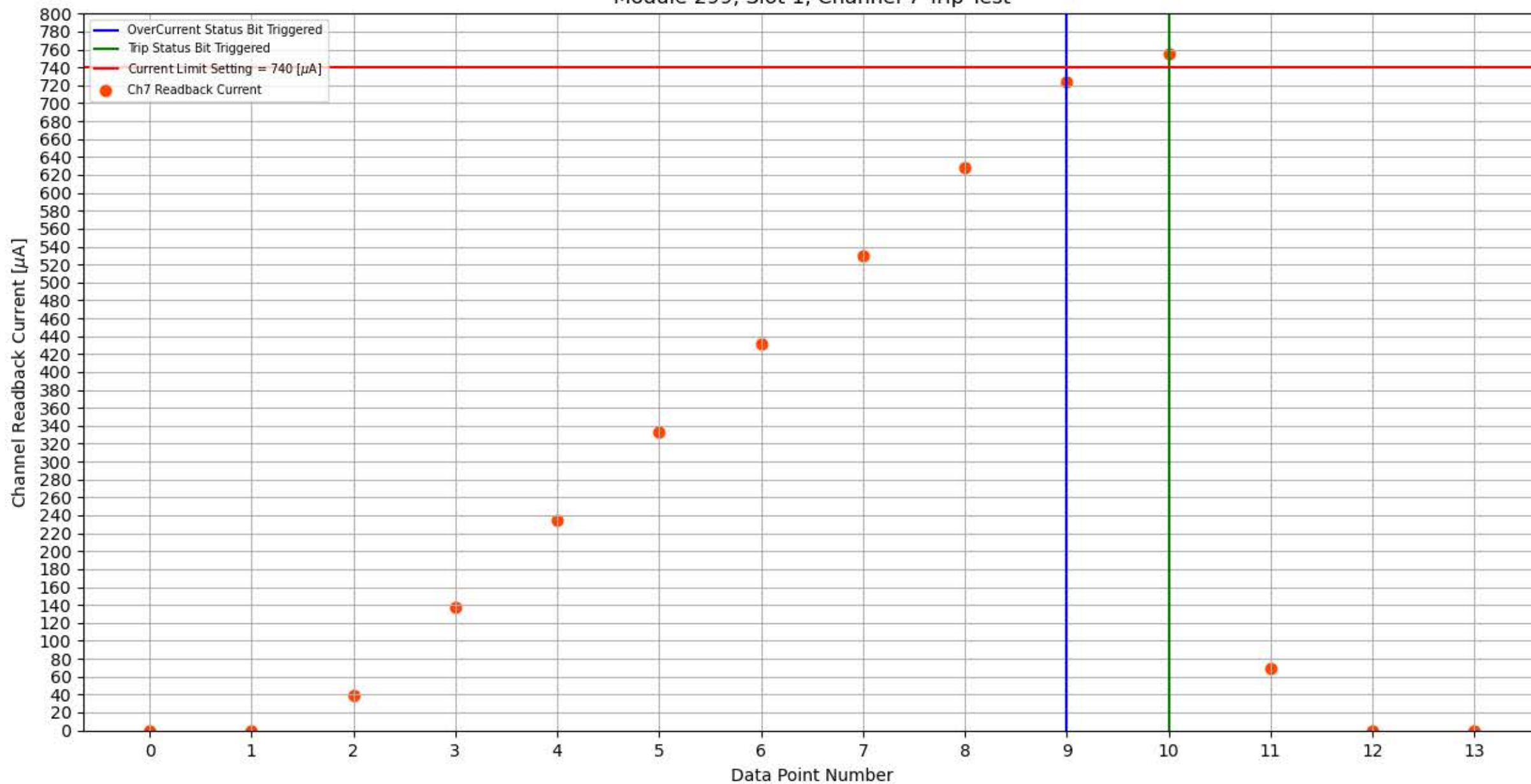
Module 299, Slot 1, Channel 7 Trip Test
