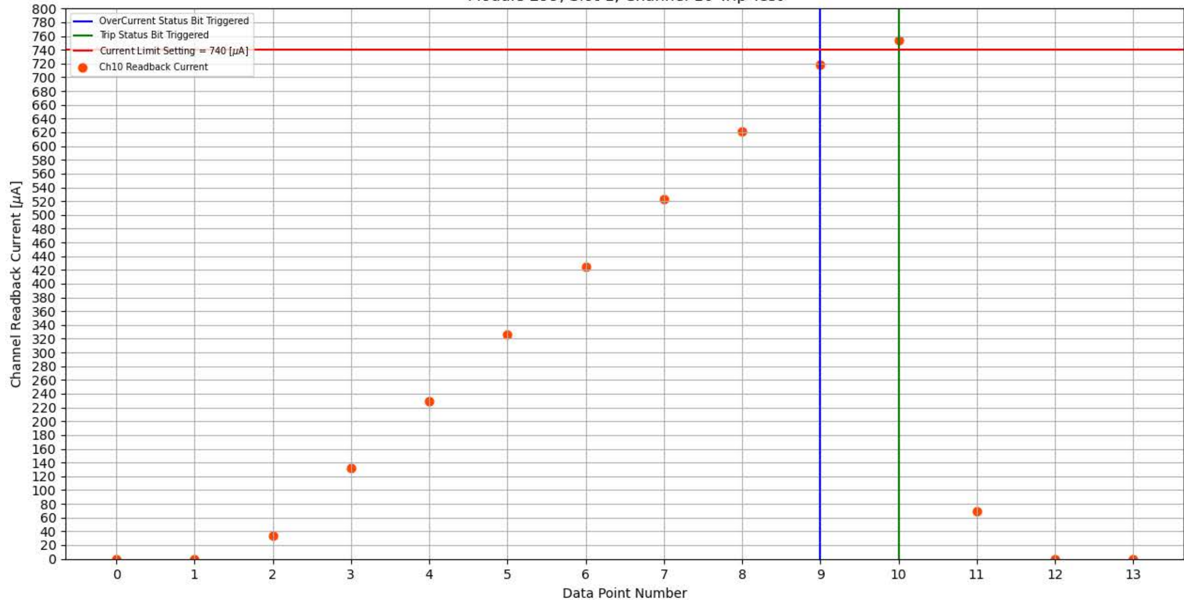
Module 299, Slot 1, Channel 10 Trip Test
