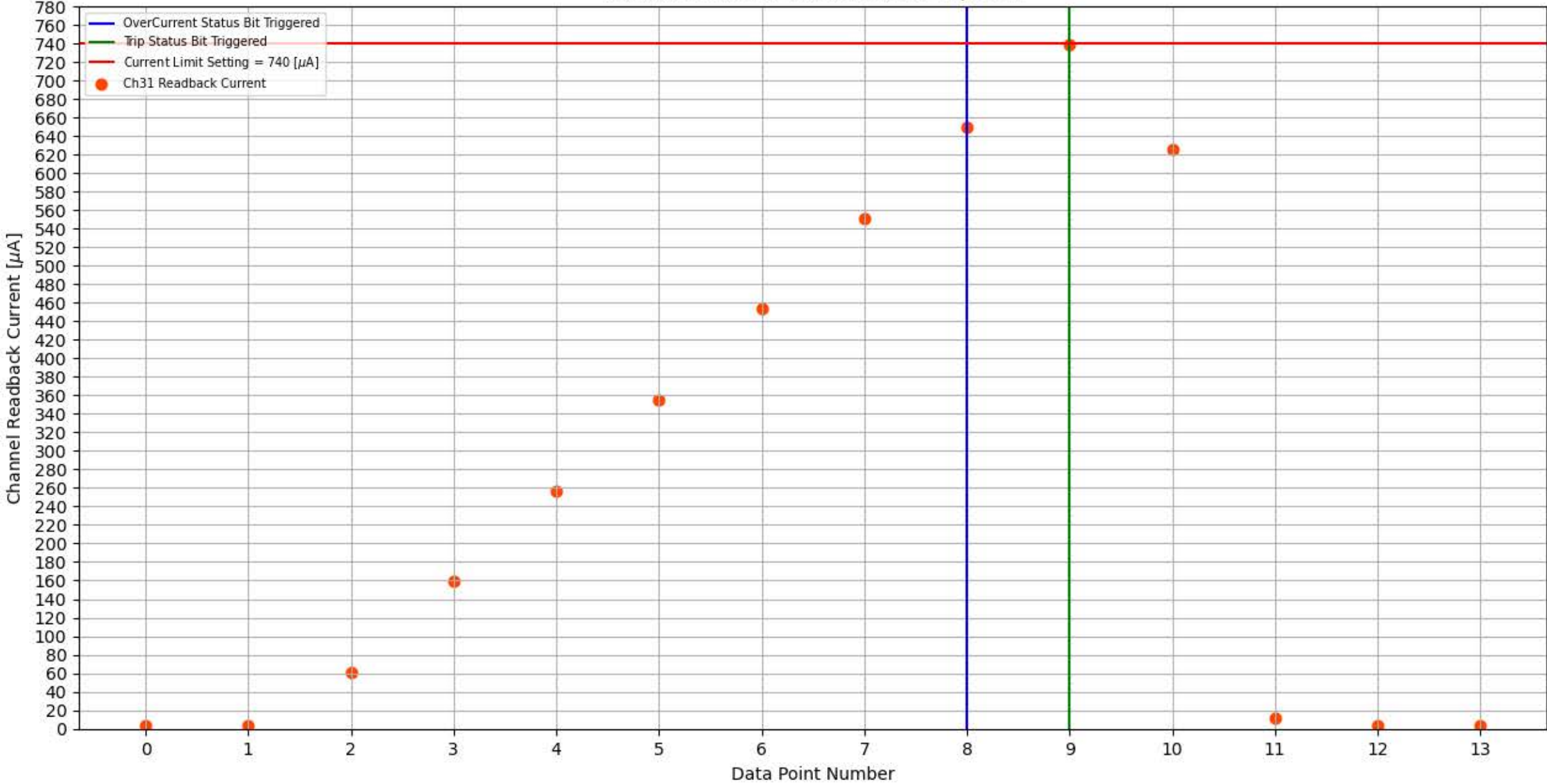
Module 299, Slot 1, Channel 31 Trip Test
