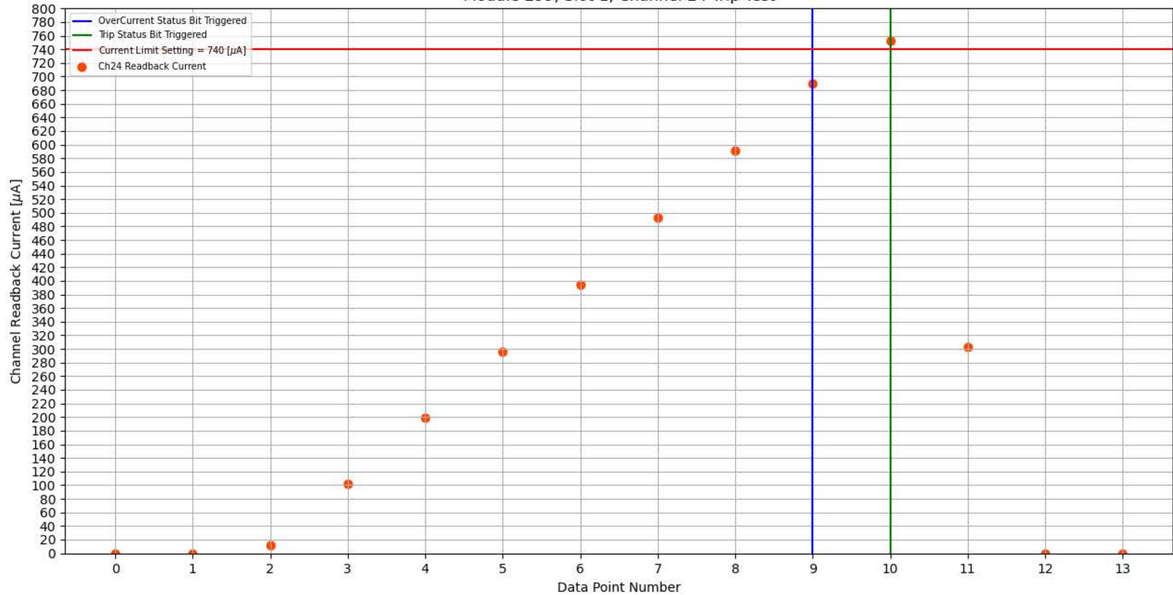
Module 299, Slot 1, Channel 24 Trip Test
