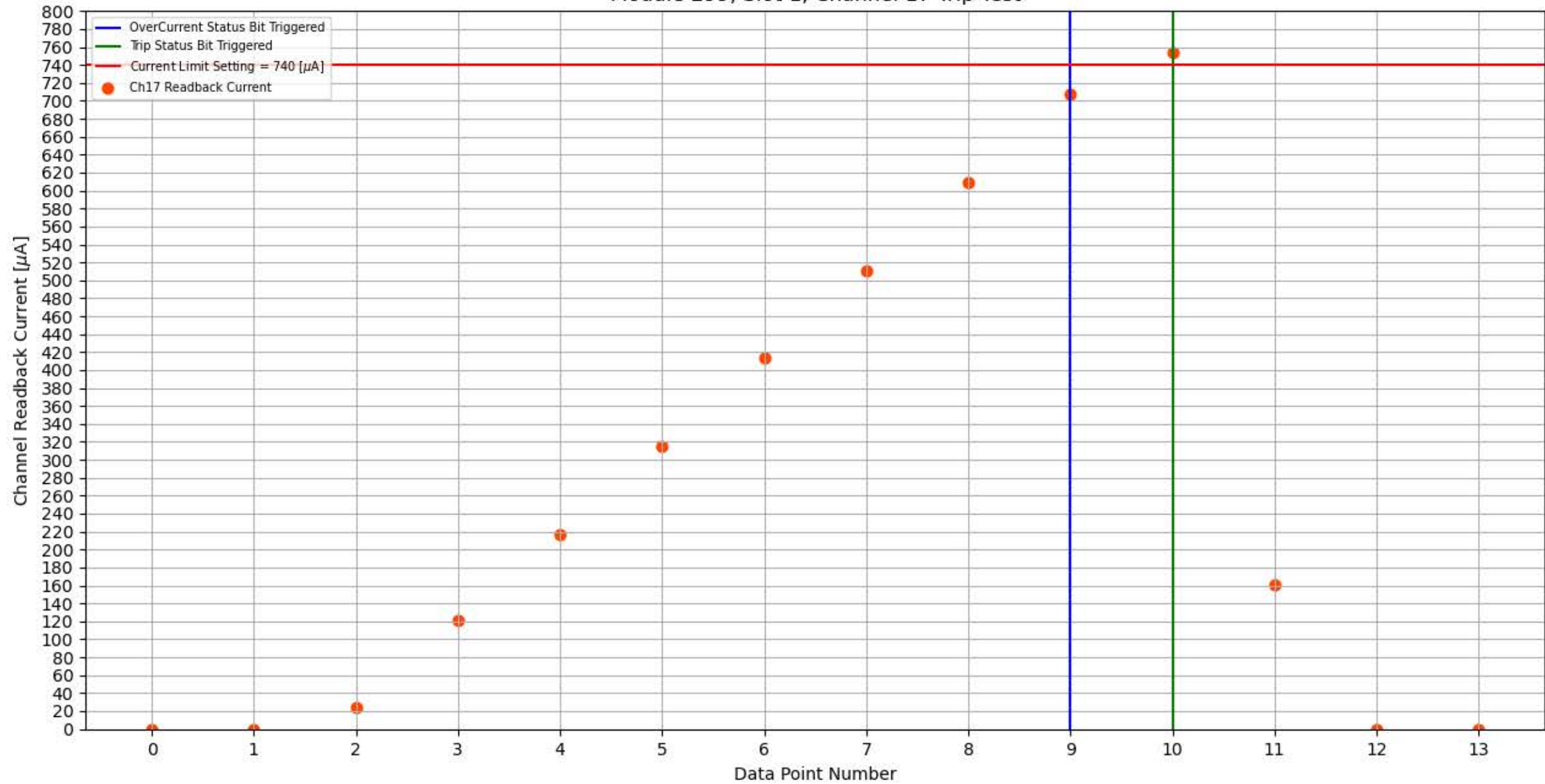
Module 299, Slot 1, Channel 17 Trip Test
