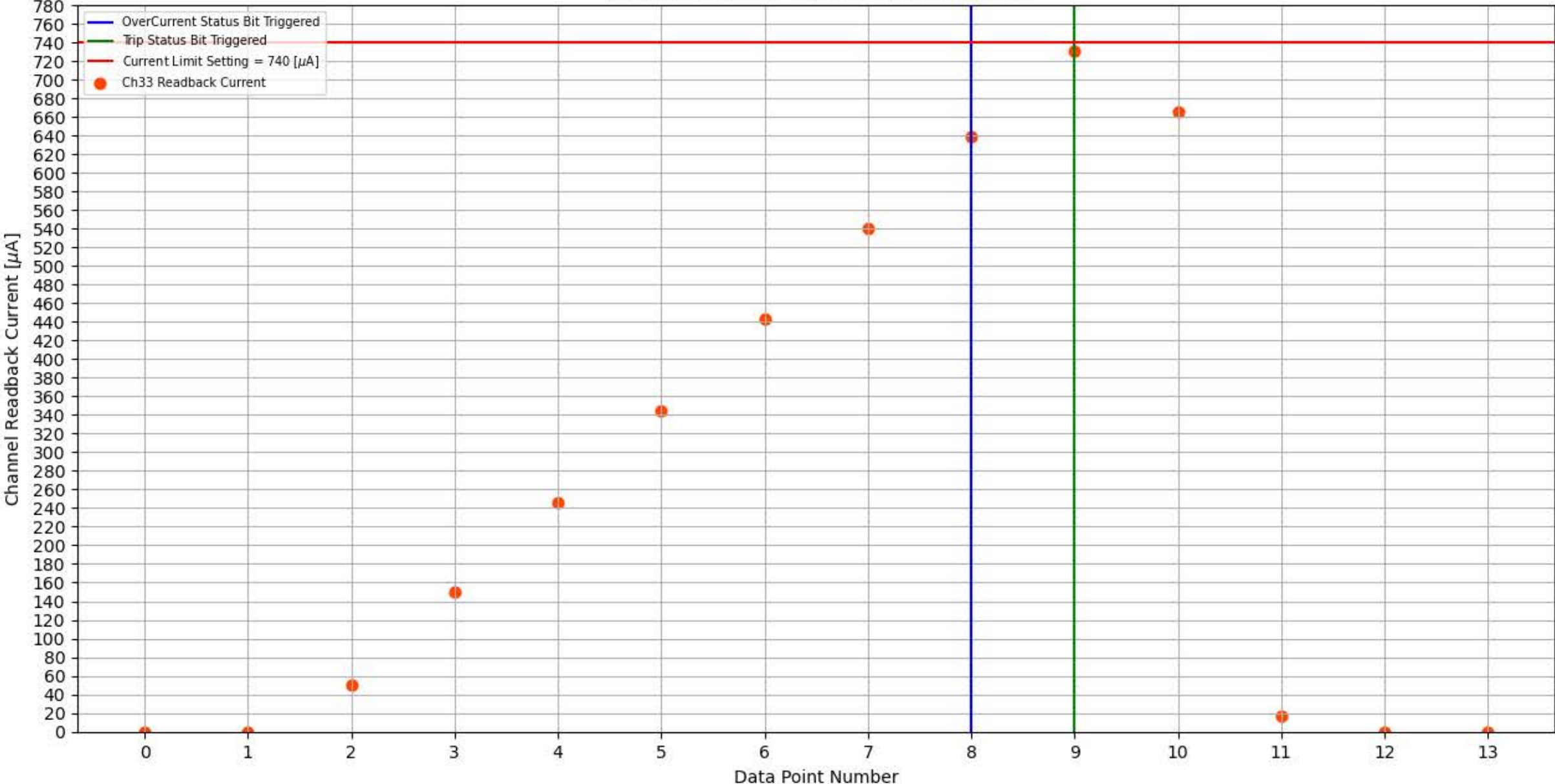
Module 299, Slot 1, Channel 33 Trip Test
