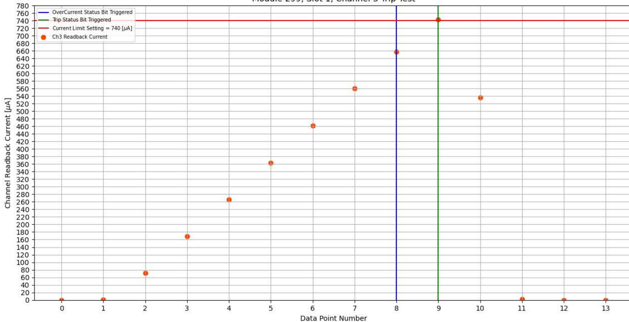
Module 299, Slot 1, Channel 3 Trip Test
