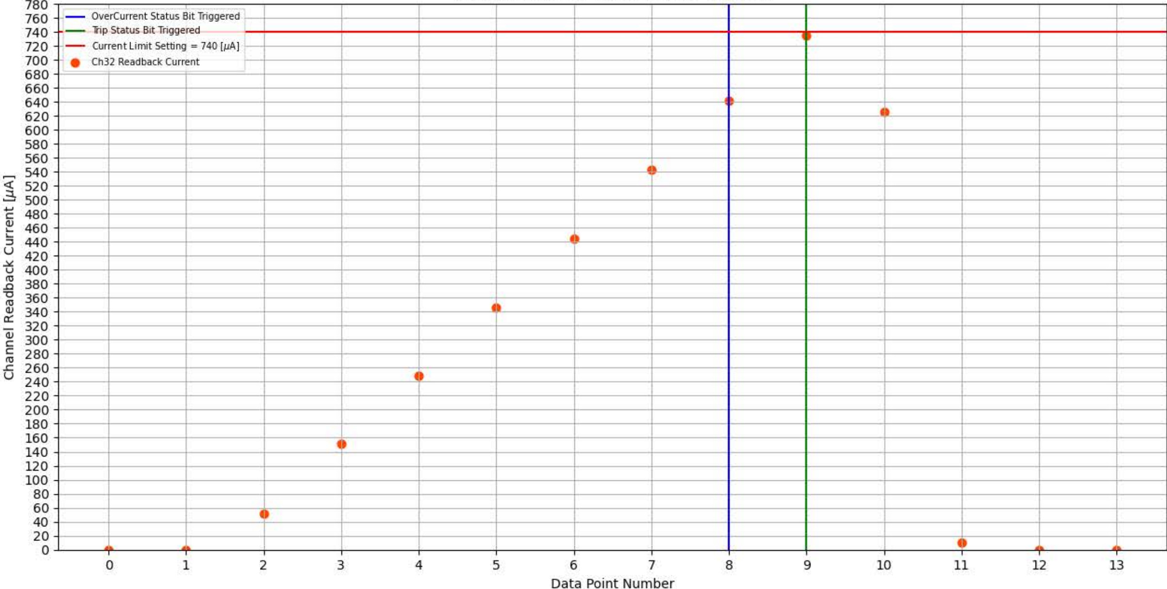
Module 299, Slot 1, Channel 32 Trip Test
