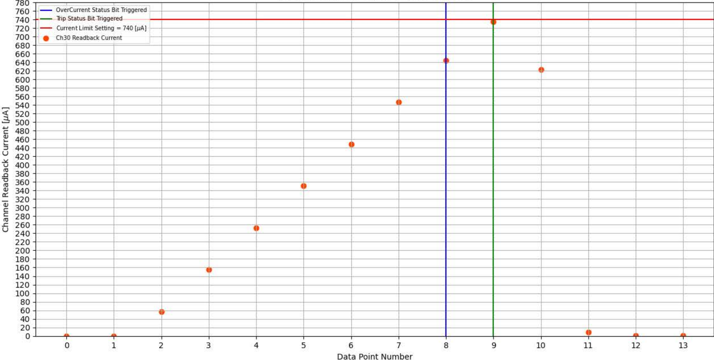
Module 299, Slot 1, Channel 30 Trip Test
