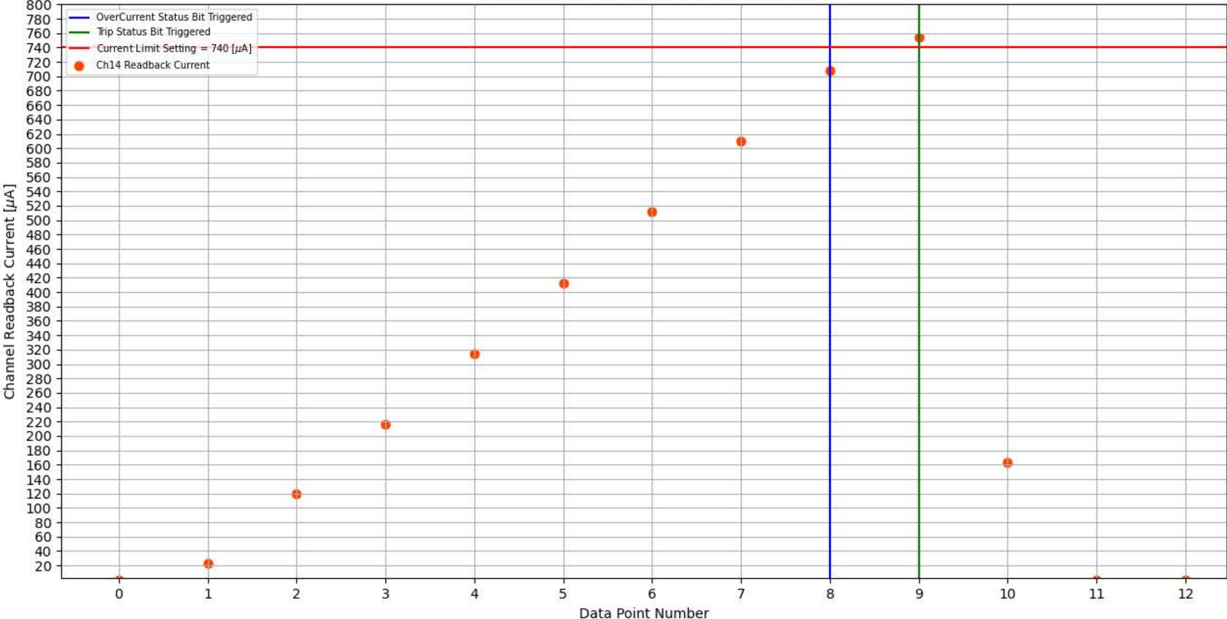
Module 299, Slot 1, Channel 14 Trip Test
