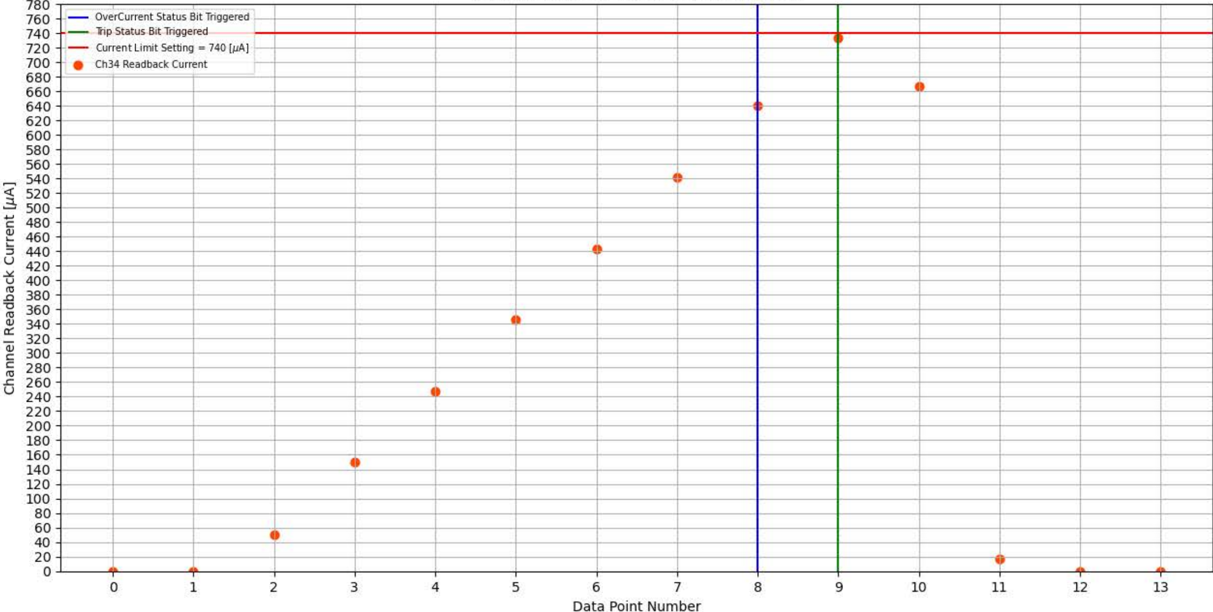
Module 299, Slot 1, Channel 34 Trip Test
