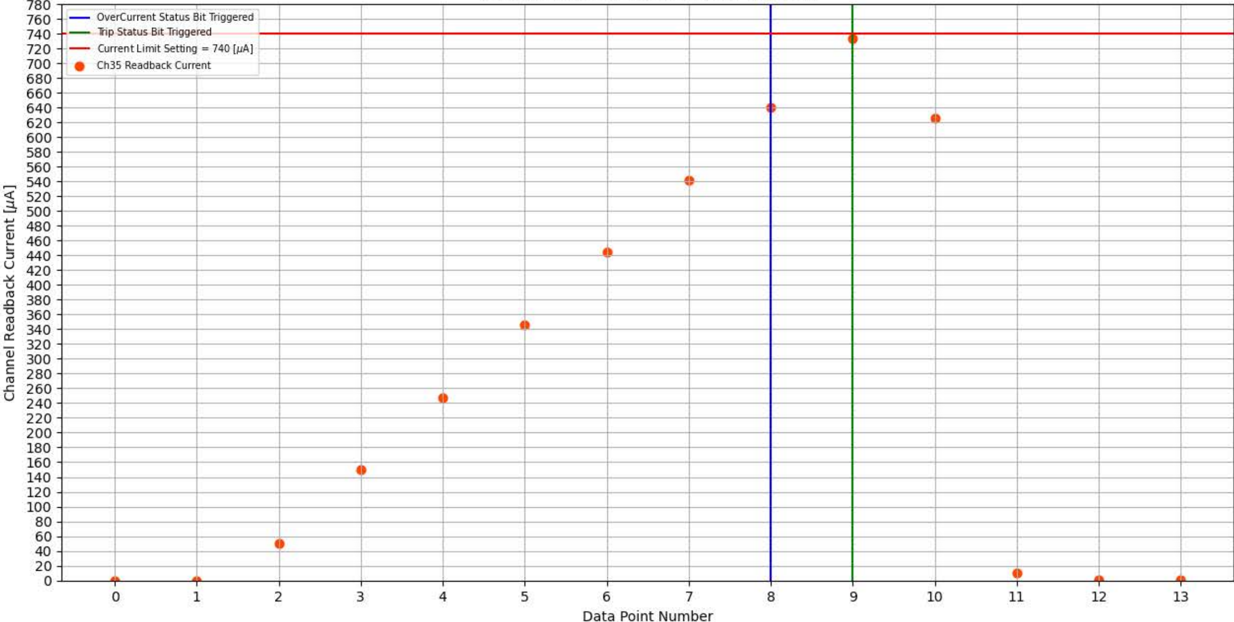
Module 299, Slot 1, Channel 35 Trip Test
