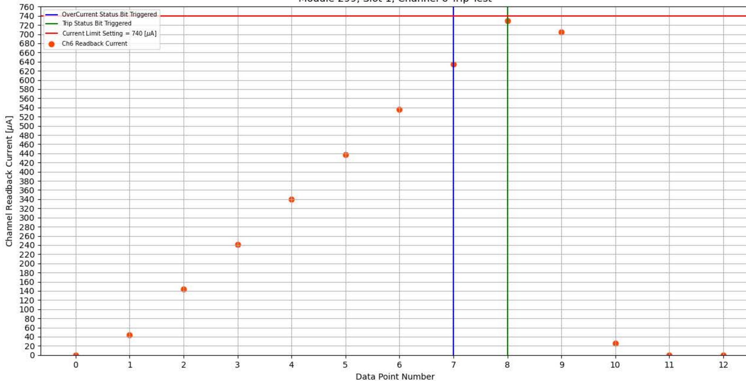
Module 299, Slot 1, Channel 6 Trip Test
