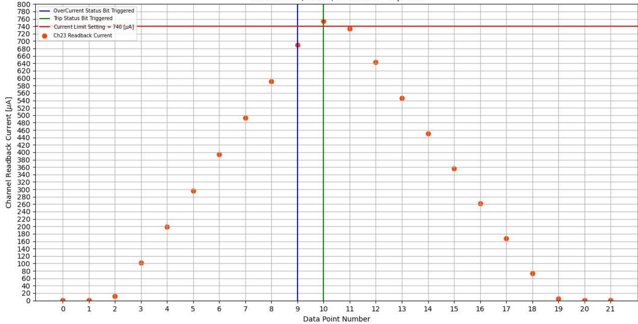
Module 299, Slot 1, Channel 23 Trip Test
