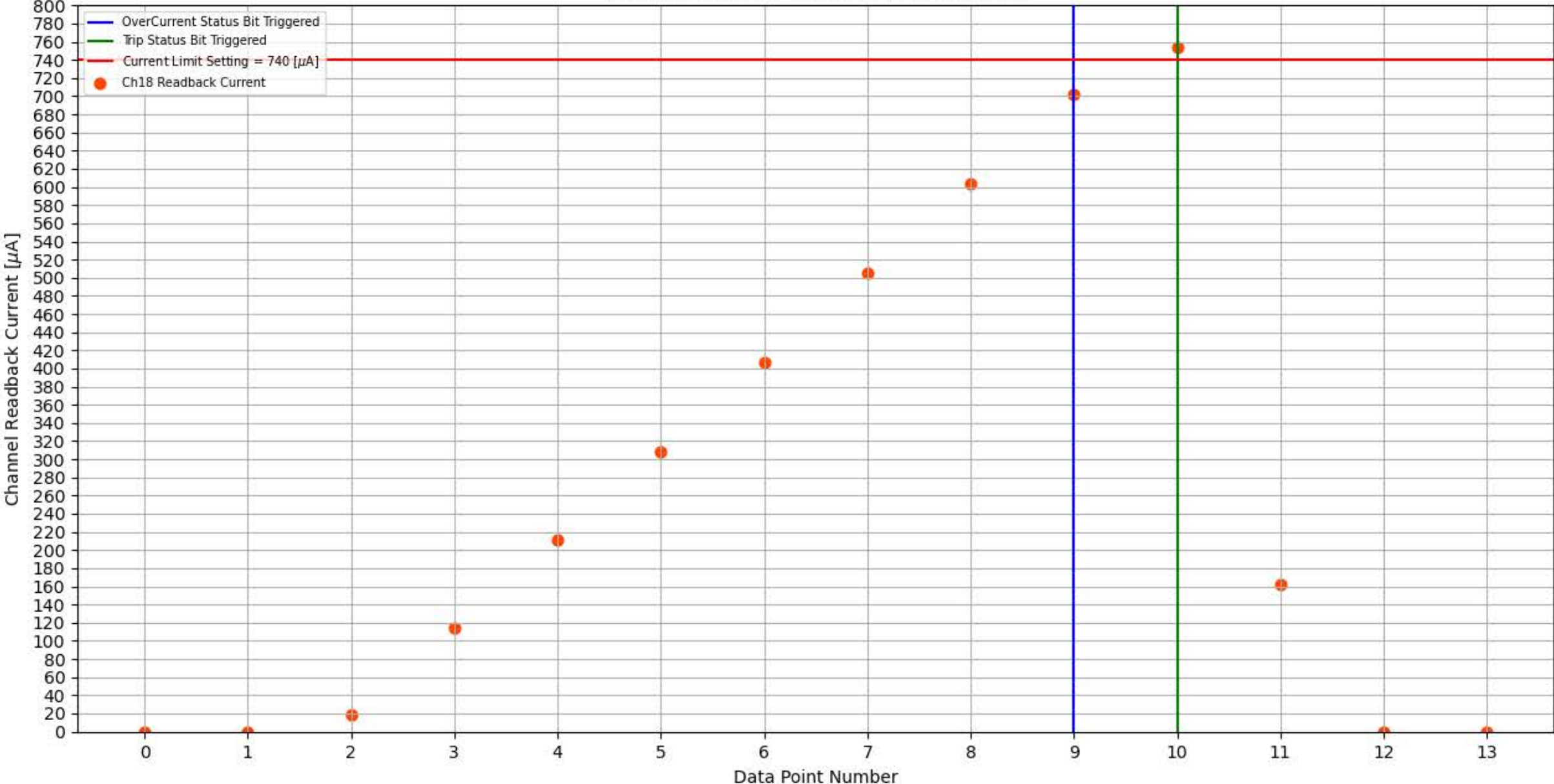
Module 299, Slot 1, Channel 18 Trip Test
