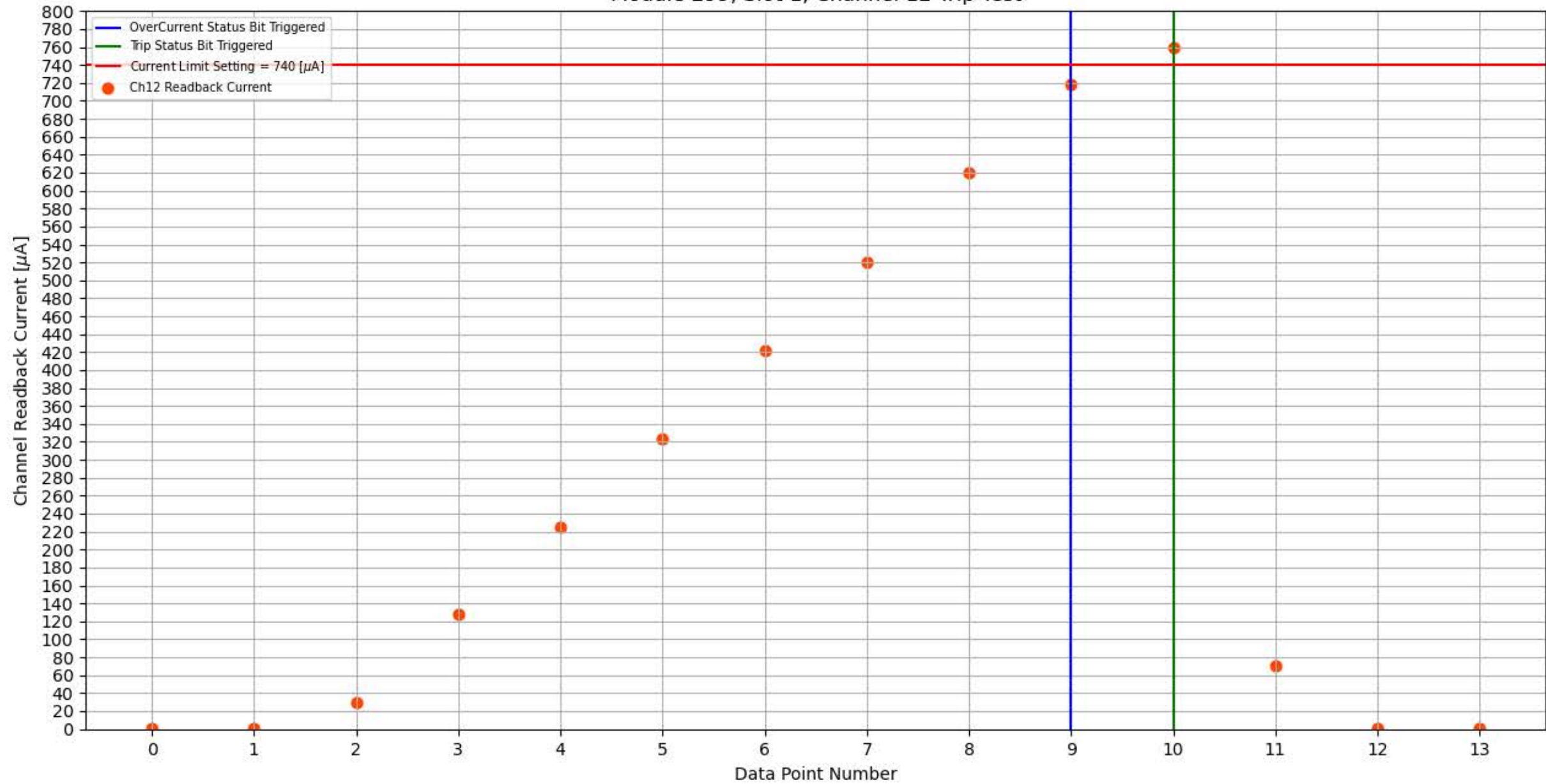
Module 299, Slot 1, Channel 12 Trip Test
