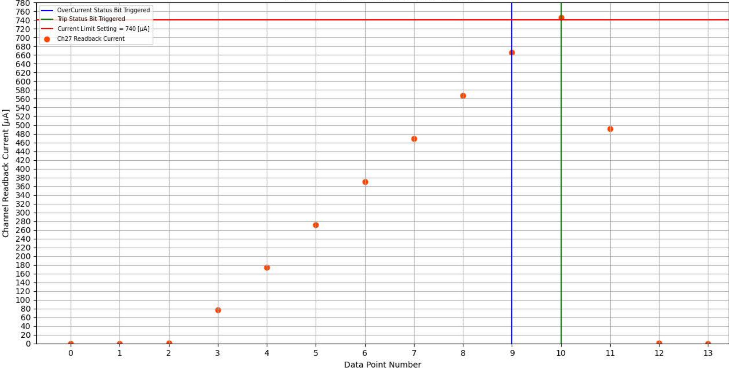
Module 299, Slot 1, Channel 27 Trip Test
