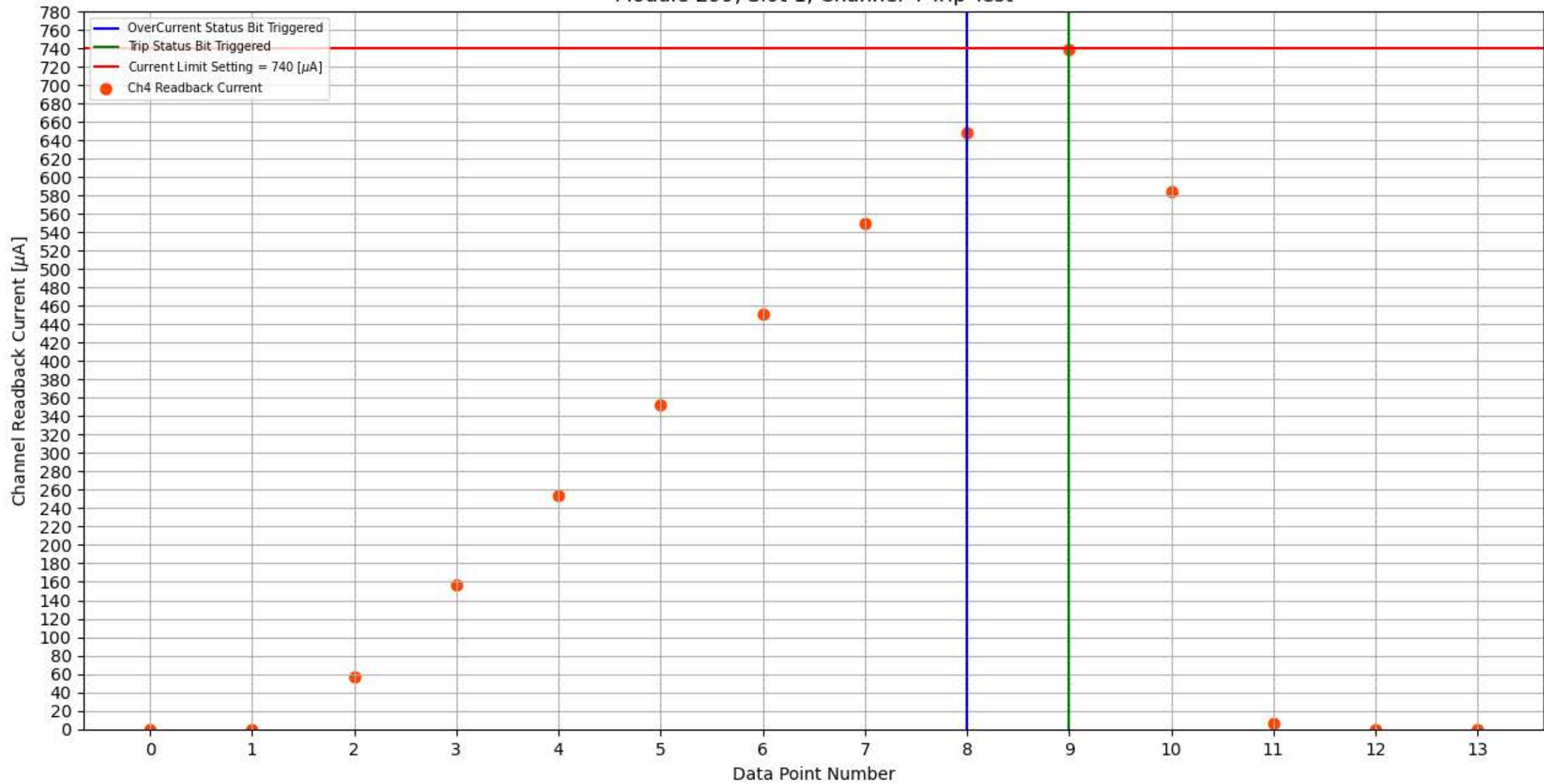
Module 299, Slot 1, Channel 4 Trip Test
