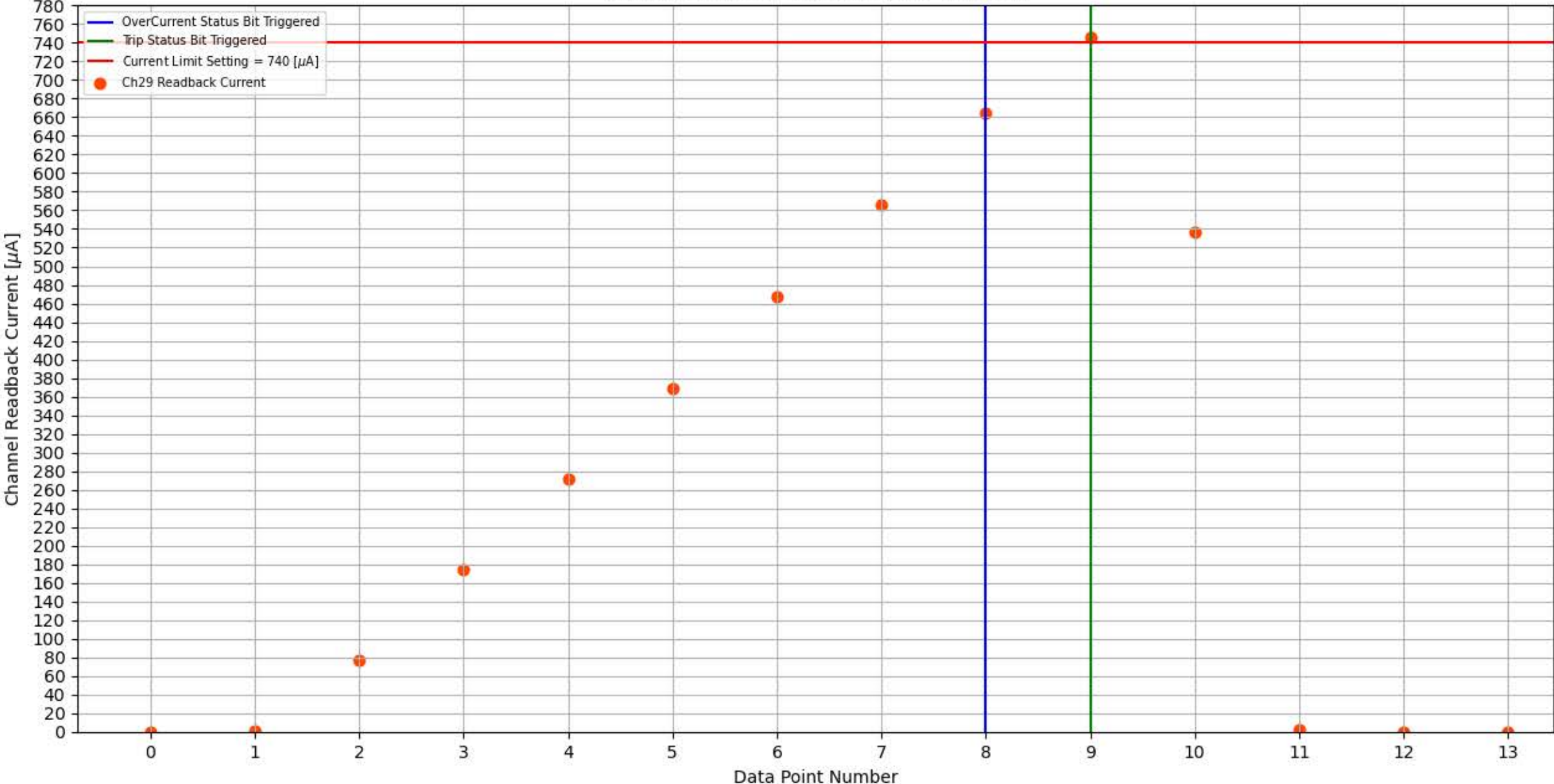
Module 299, Slot 1, Channel 29 Trip Test
