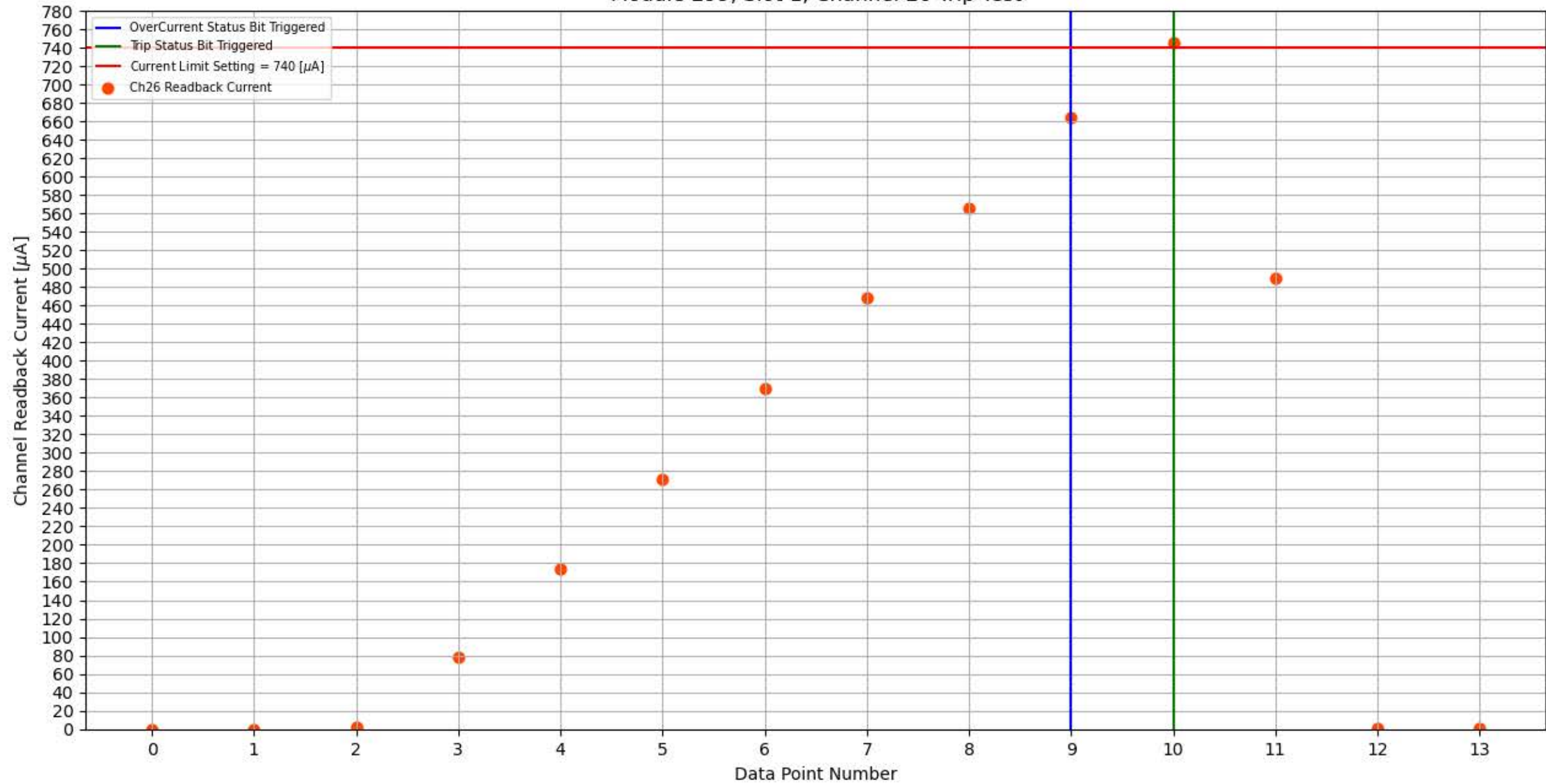
Module 299, Slot 1, Channel 26 Trip Test
