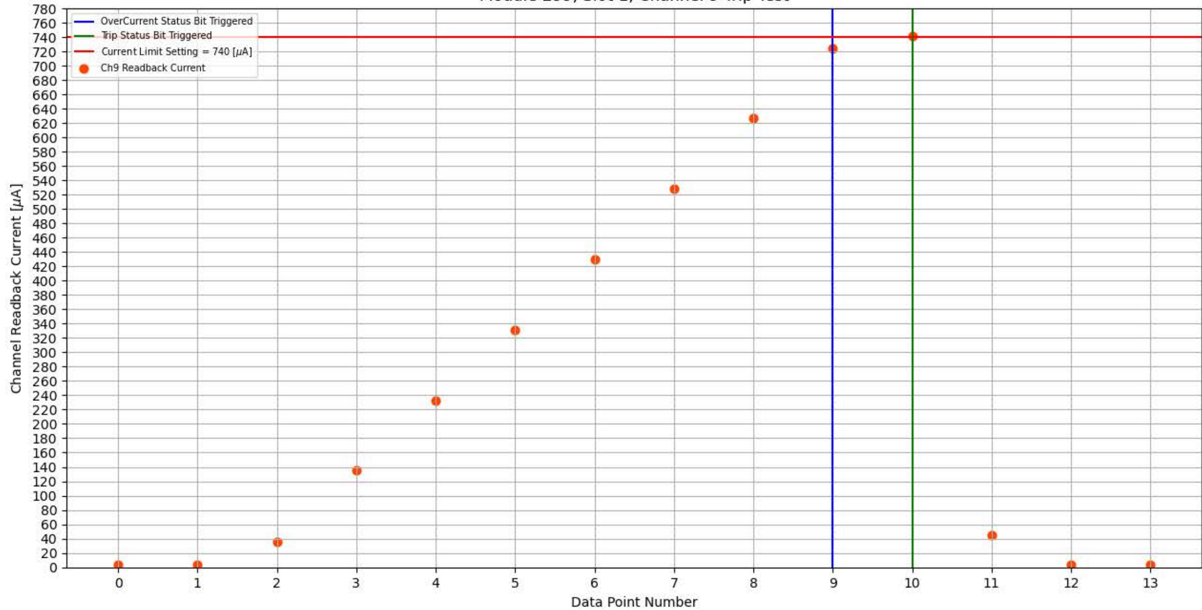
Module 299, Slot 1, Channel 9 Trip Test
