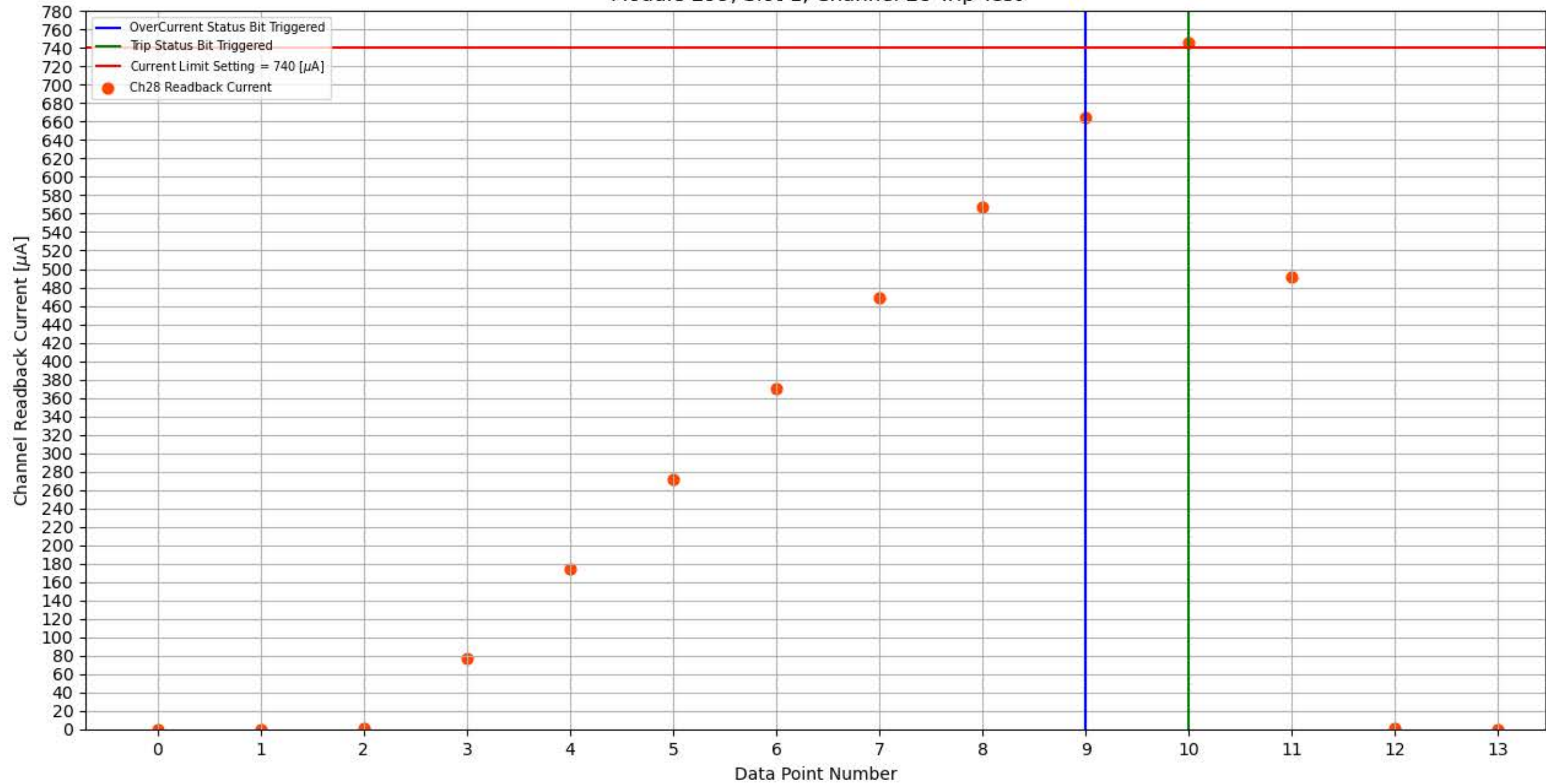
Module 299, Slot 1, Channel 28 Trip Test
