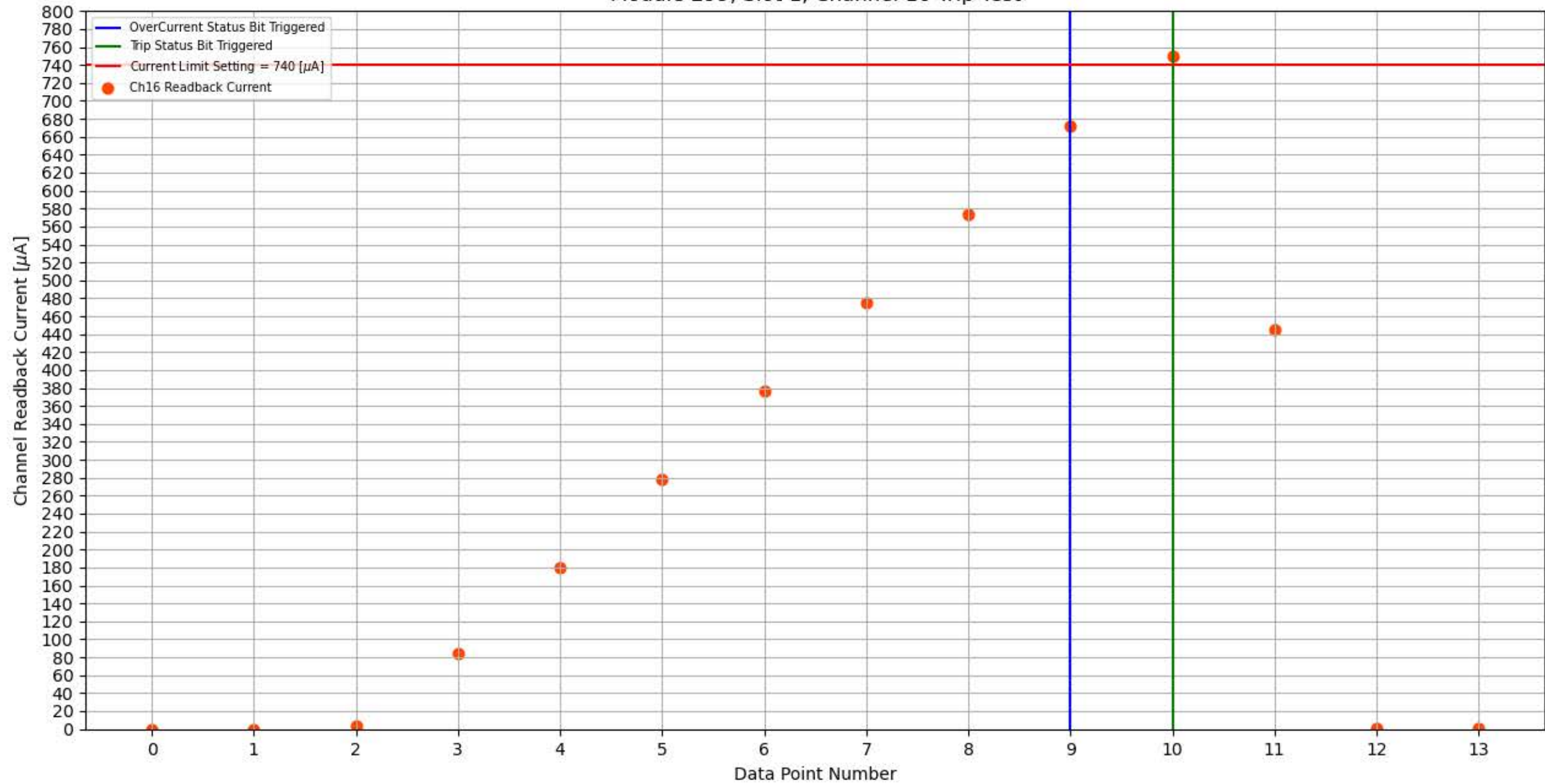
Module 299, Slot 1, Channel 16 Trip Test
