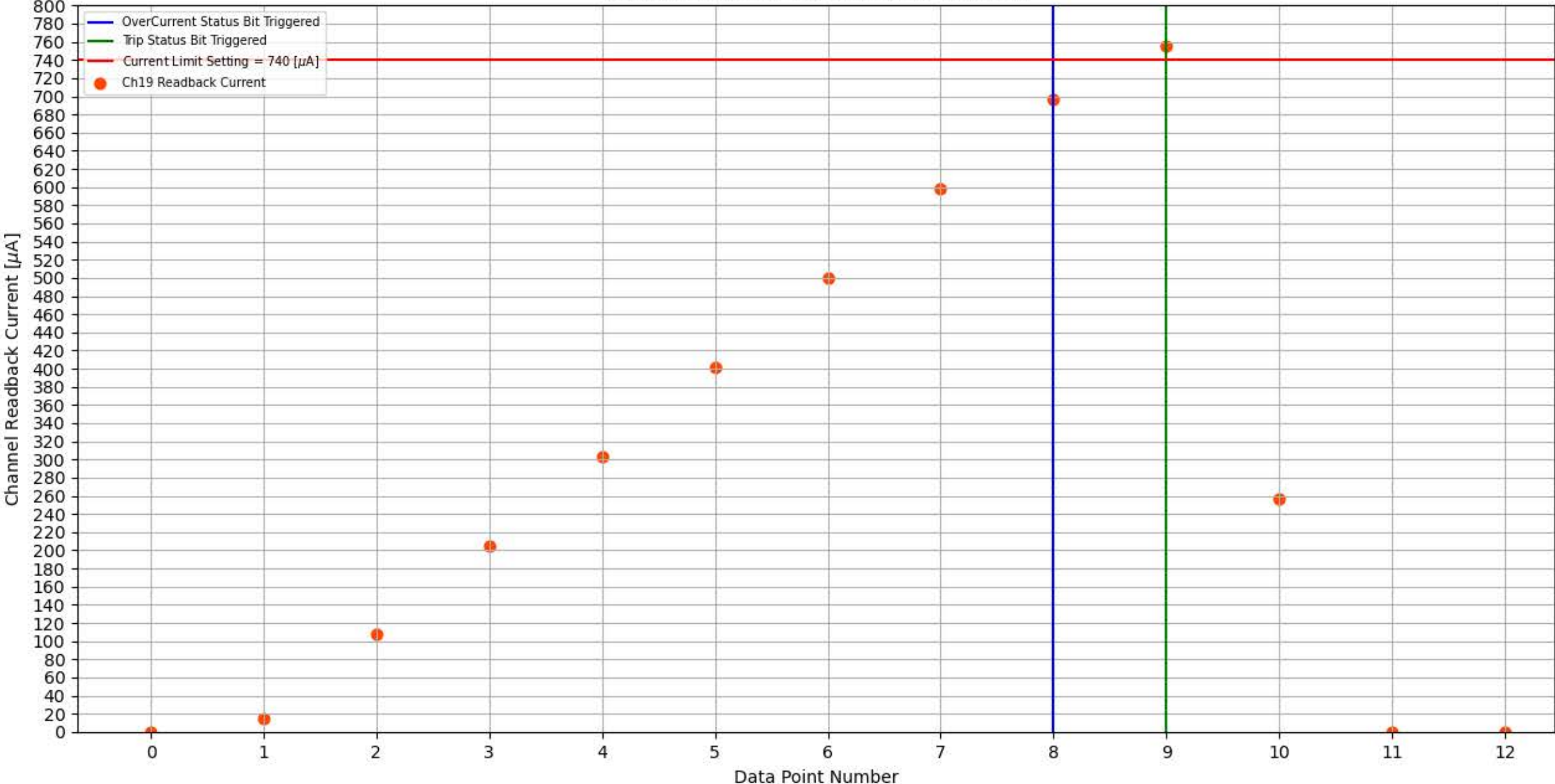
Module 299, Slot 1, Channel 19 Trip Test
