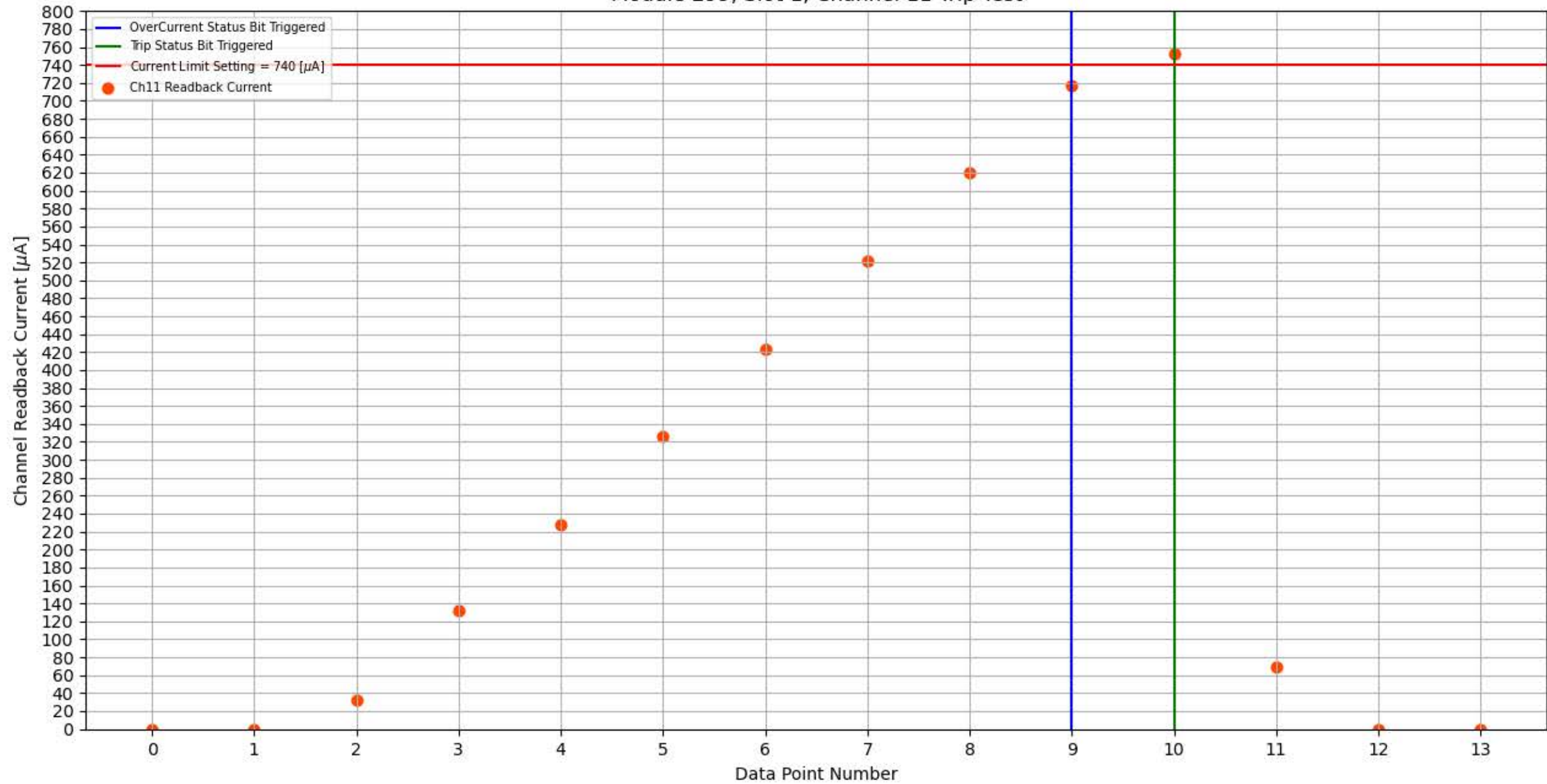
Module 299, Slot 1, Channel 11 Trip Test
