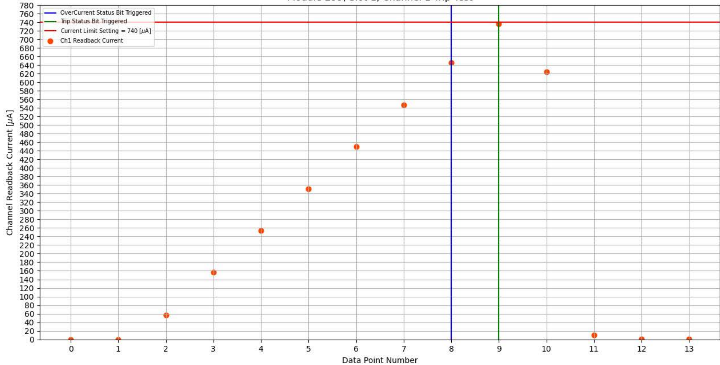
Module 299, Slot 1, Channel 1 Trip Test
