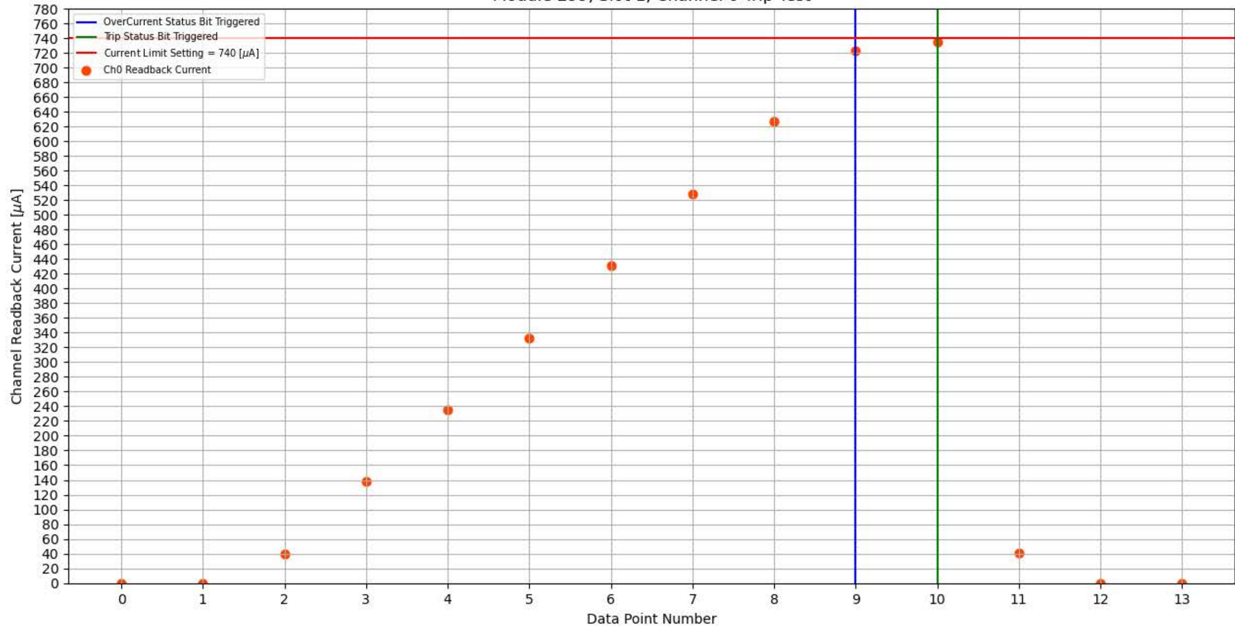
Module 299, Slot 1, Channel 0 Trip Test
