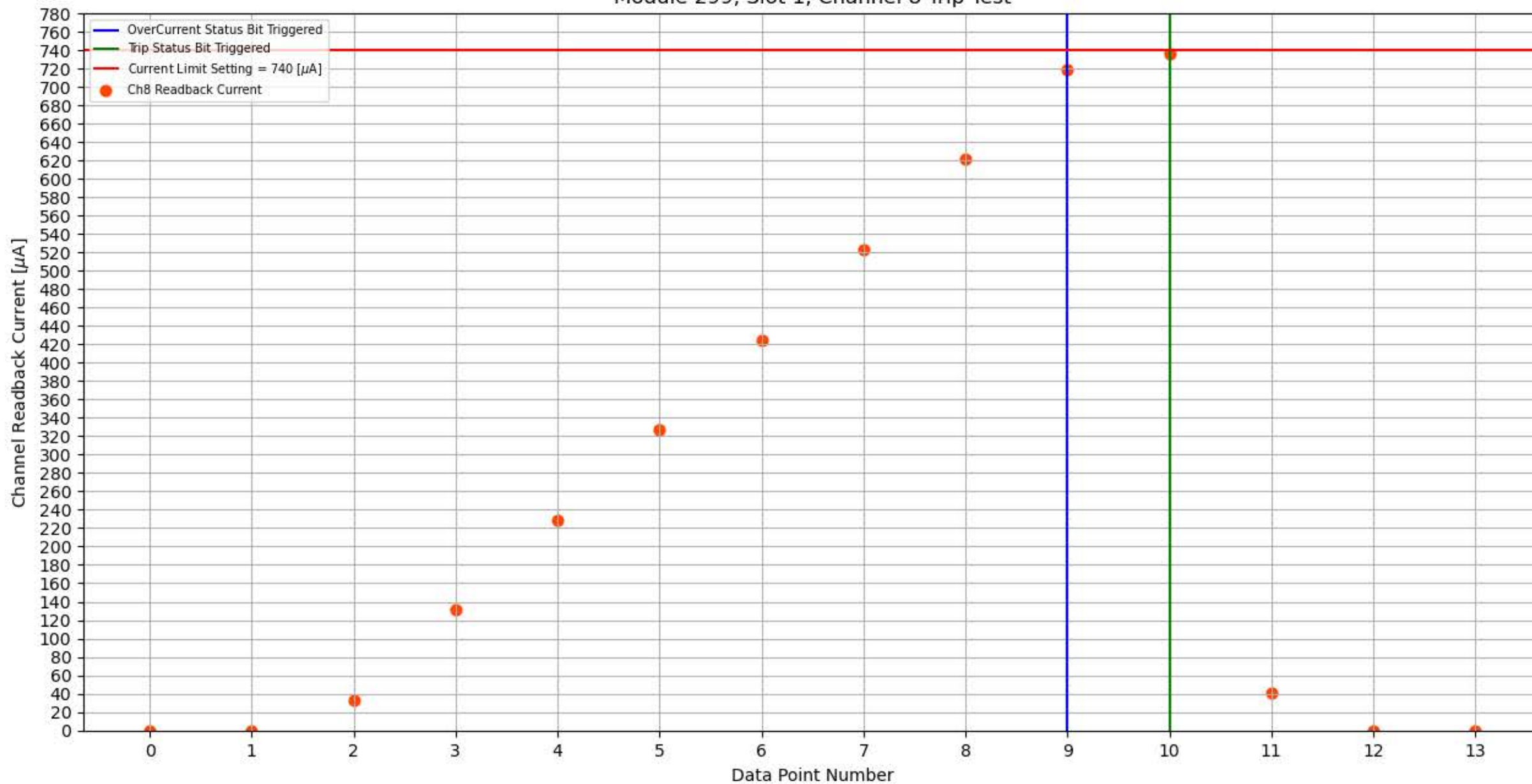
Module 299, Slot 1, Channel 8 Trip Test
