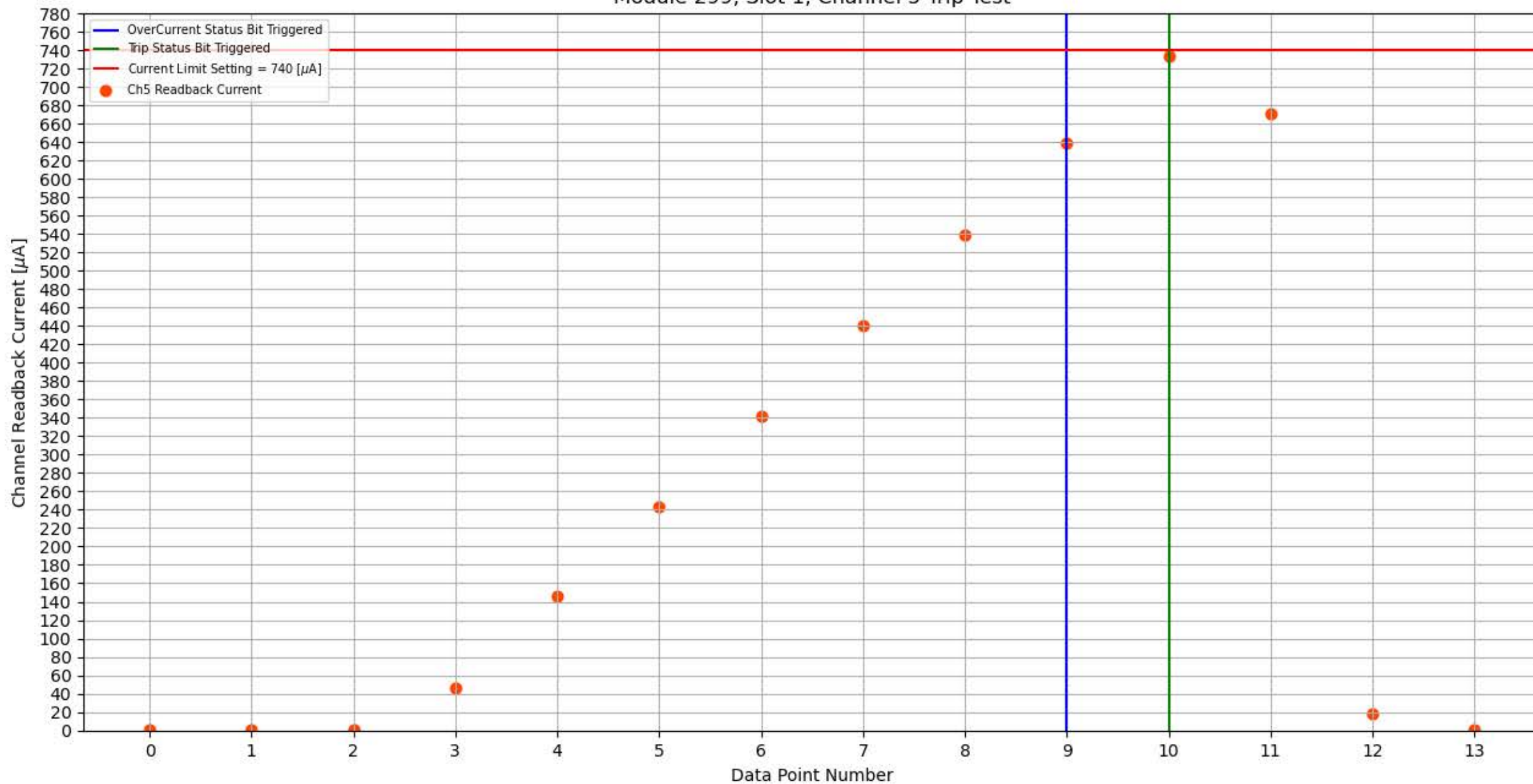
Module 299, Slot 1, Channel 5 Trip Test
