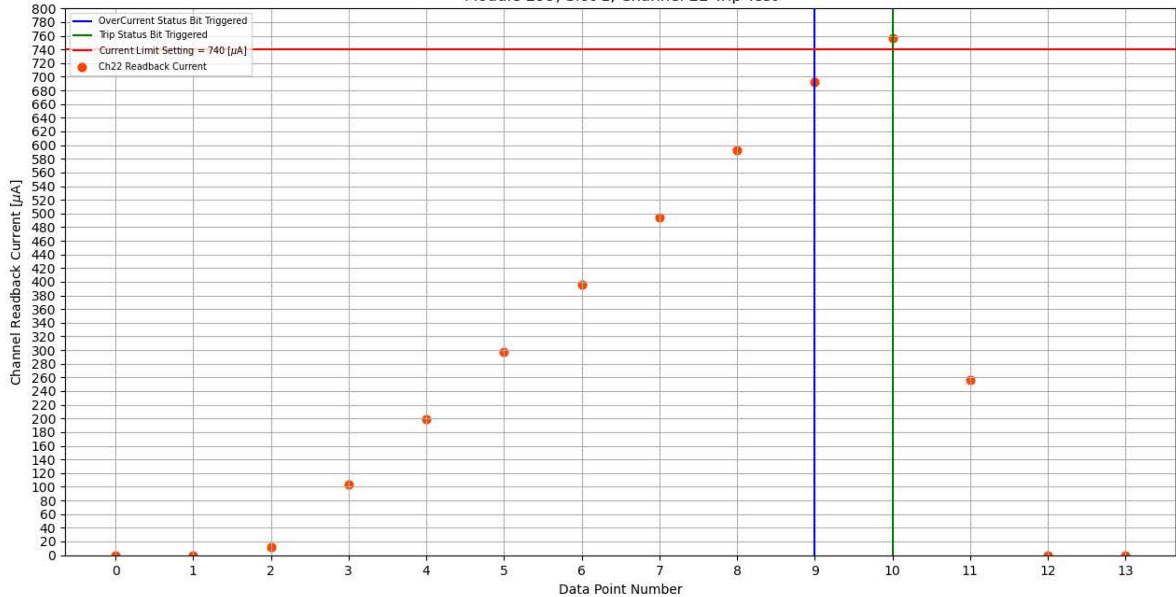
Module 299, Slot 1, Channel 22 Trip Test
