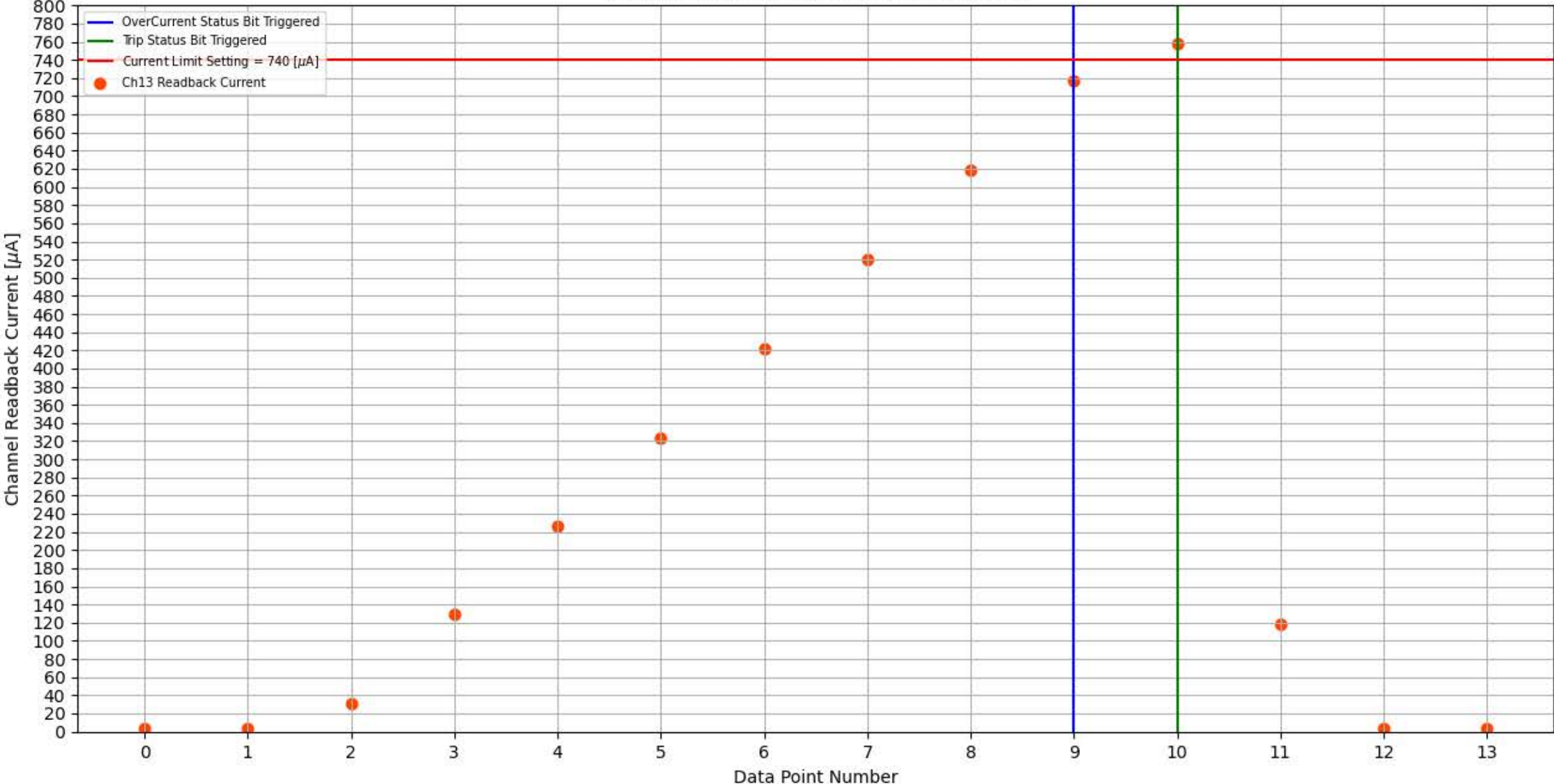
Module 299, Slot 1, Channel 13 Trip Test
